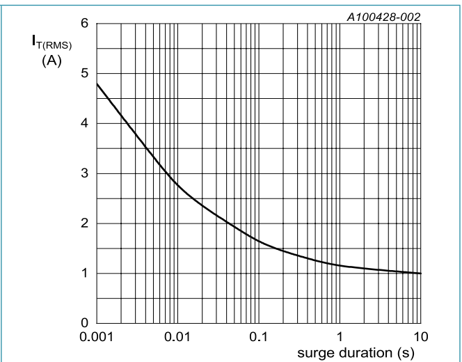
f = 50\text{ Hz} ; T_{sp} = 121\text{ }^{\circ}\text{C} Fig. 2. RMS on-state current as a function of surge duration; maximum values
